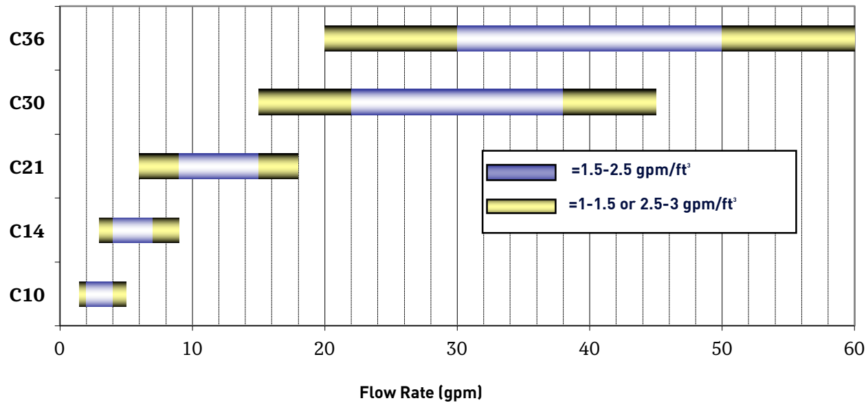
Figure 1. E-Series Activated Carbon Flow Range
