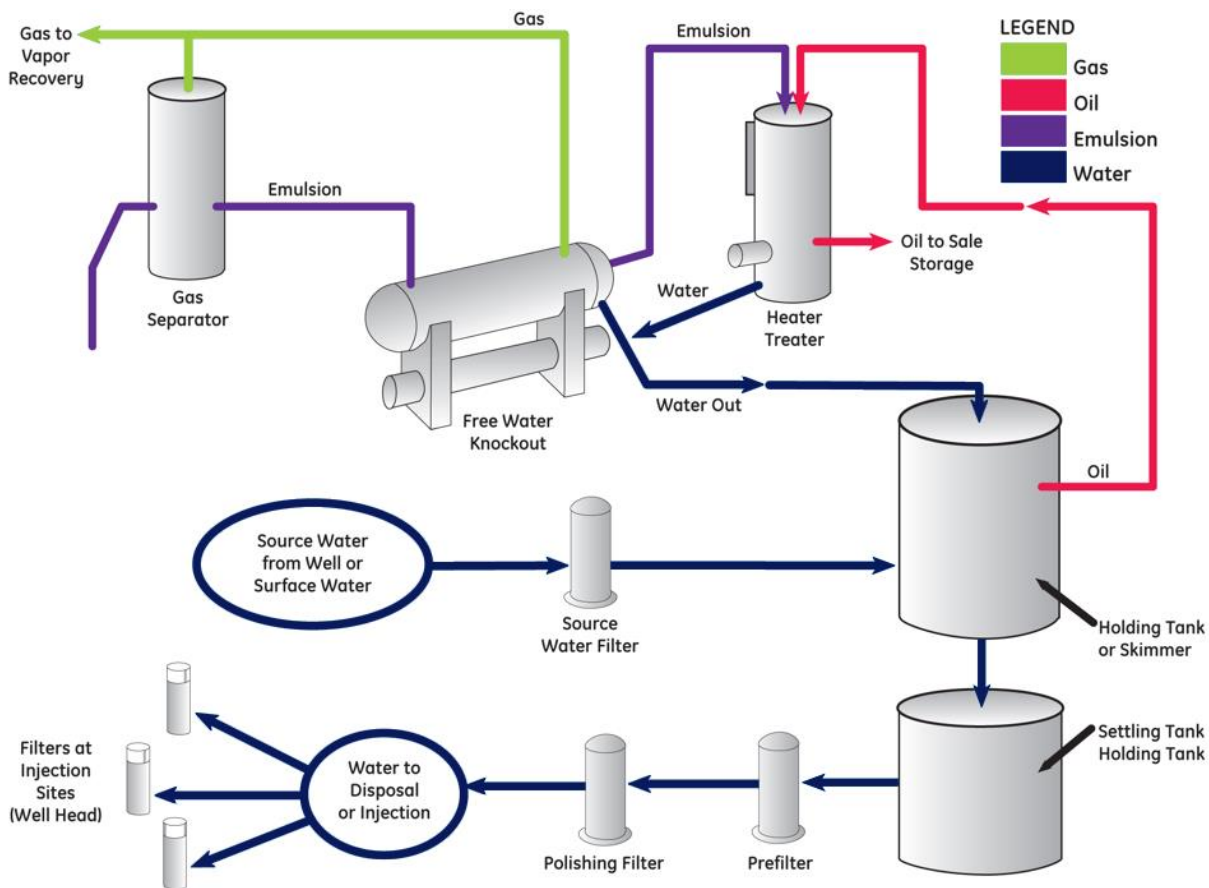
Figure 1: Filter Applications for Water Flood Systems Schematic
