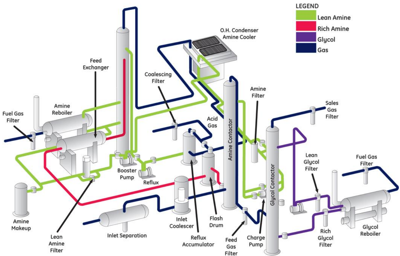
Figure 1: Filter Applications for Natural Gas Processing Schematic
